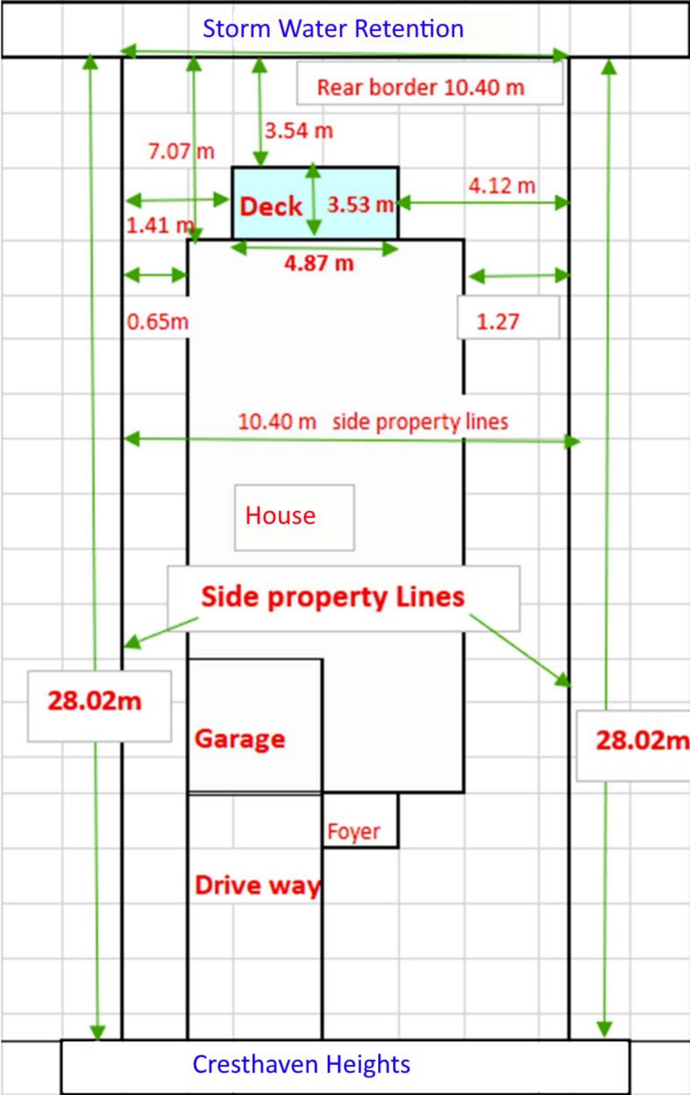
Figure 1 Site sketch showing dimensions of current deck, highlighted, and setbacks to property lines.
