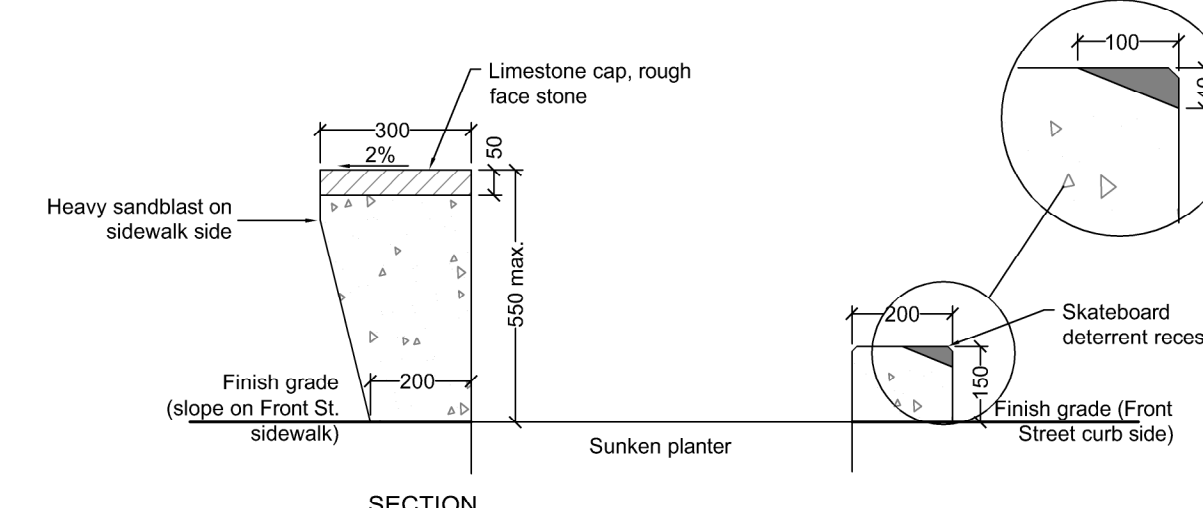
1 SEATWALL AND CURB WALL 1:15
