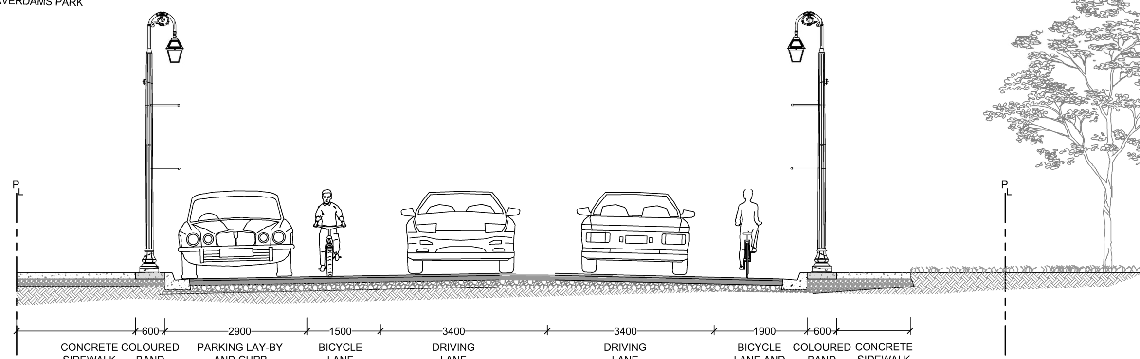
SECTION B-B, SULLIVAN AVENUE 1:75
