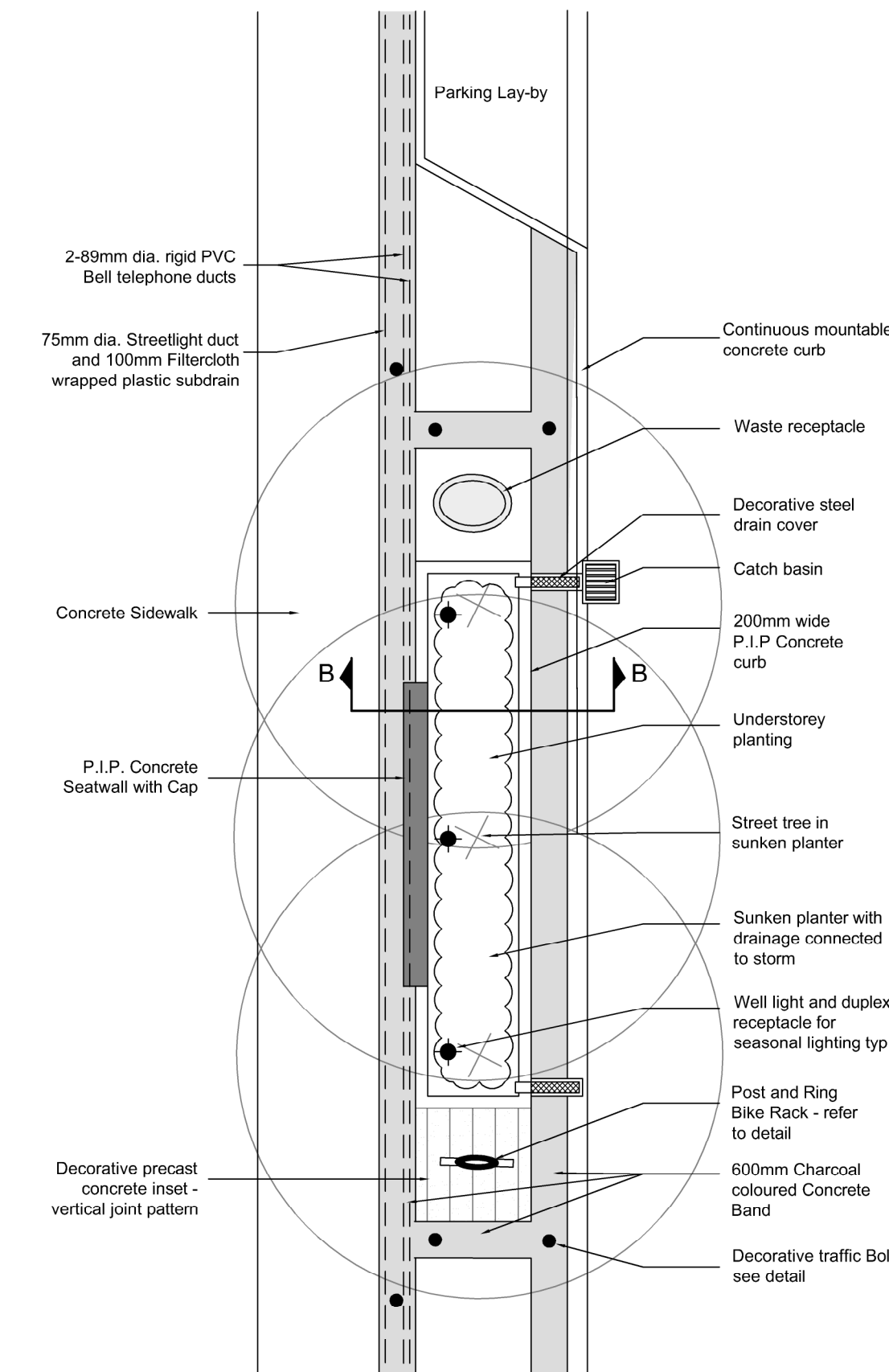
2 SUNKEN PLANTER/SEATWALL ENLARGEMENT - PLAN 1:100
