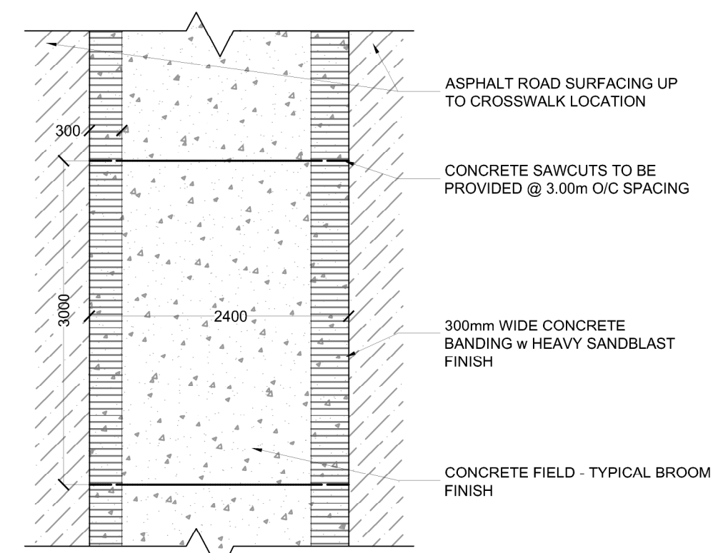
2 CROSSWALK PAVING - TYPICAL DETAIL - 2.40m WIDTH 1:50
