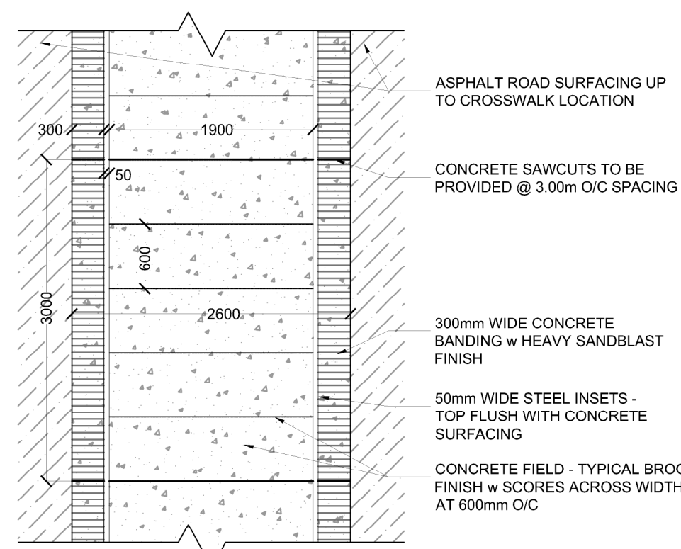
1 CROSSWALK PAVING - FRONT STREET - 2.60m WIDTH 1:50
