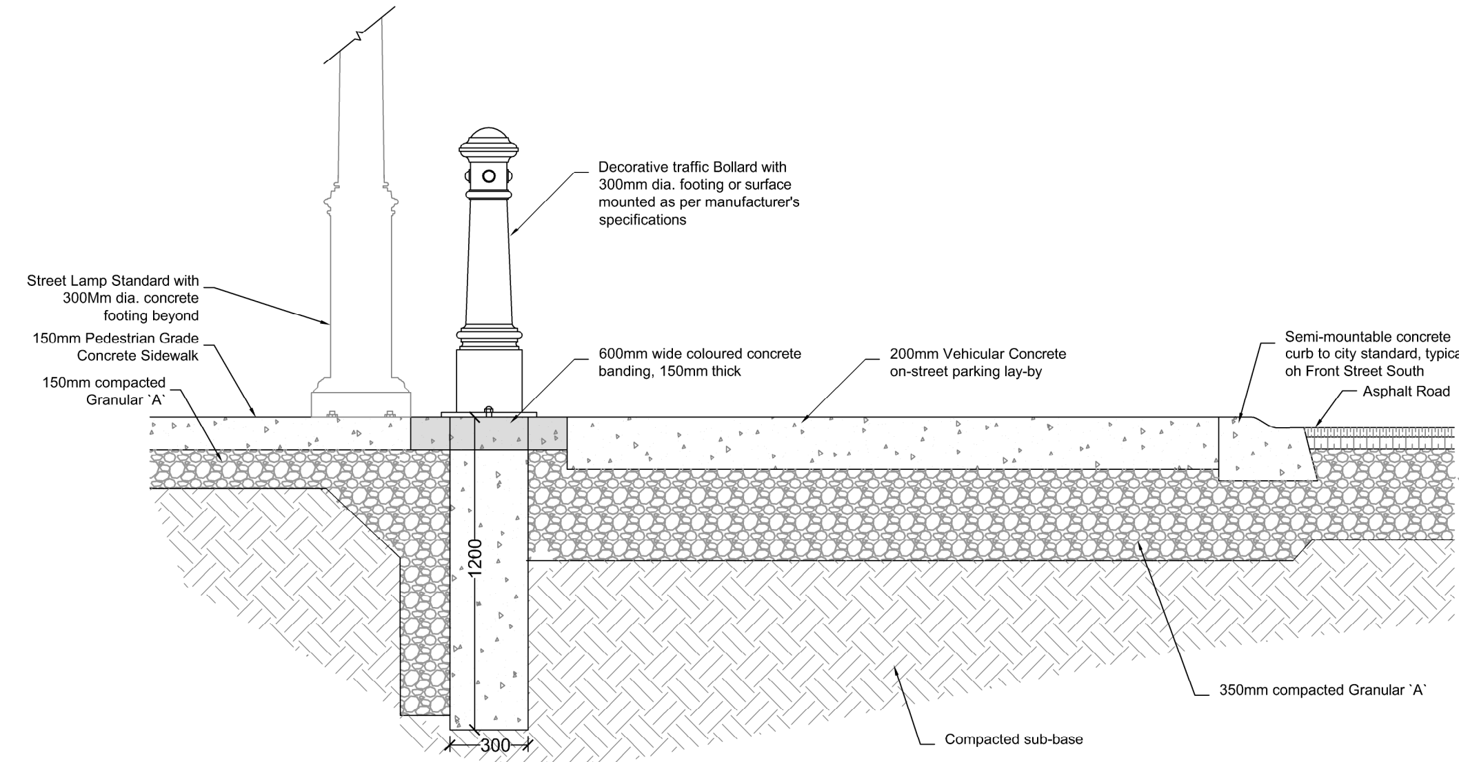
SECTION A-A FRONT STREET SOUTH AT PARKING LAY-BY 1:20
