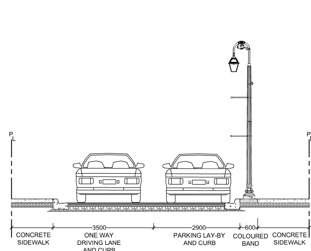
SECTION B-B, ALBERT STREET EAST 1:75
